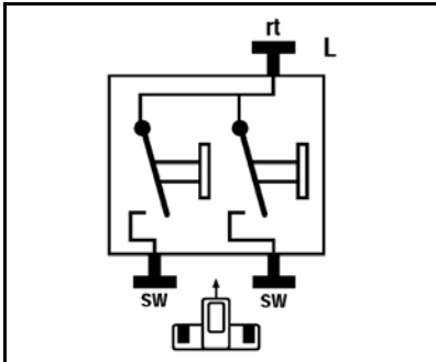
Contact assignments
