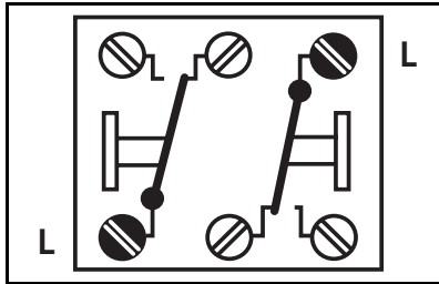
Contact assignments
