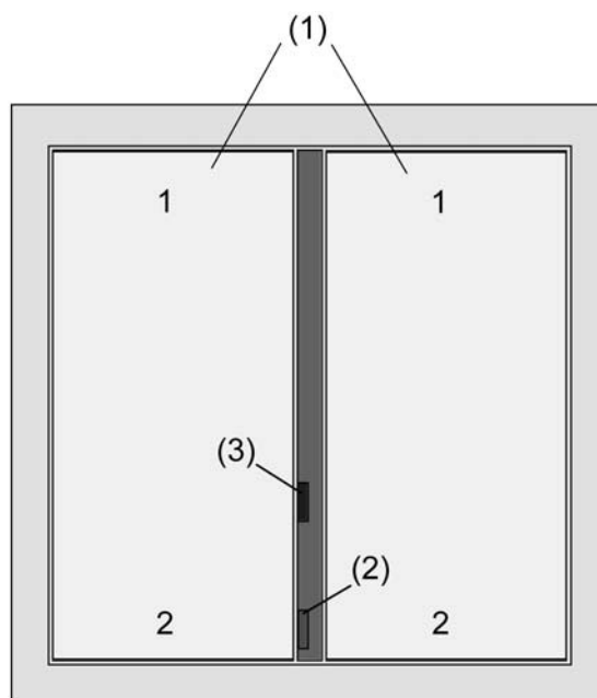
picture 1: Device arrangement of the 1-gang Standard TSM push button sensor
