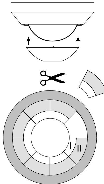
Figure 11: Push-on cover
