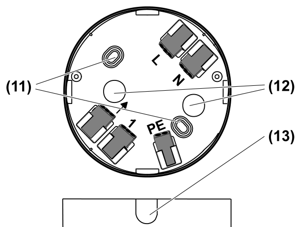
Figure 8: Connection box
